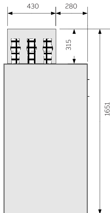
Busbar cover
