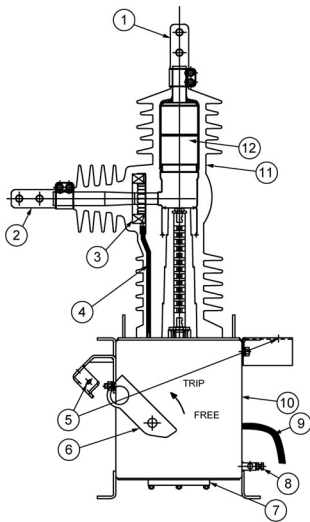
Cross section of E series 27 kV switchgear
