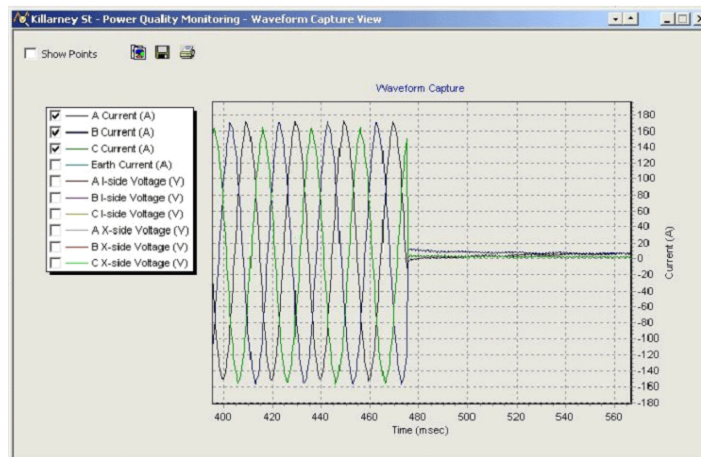
Waveform capture
