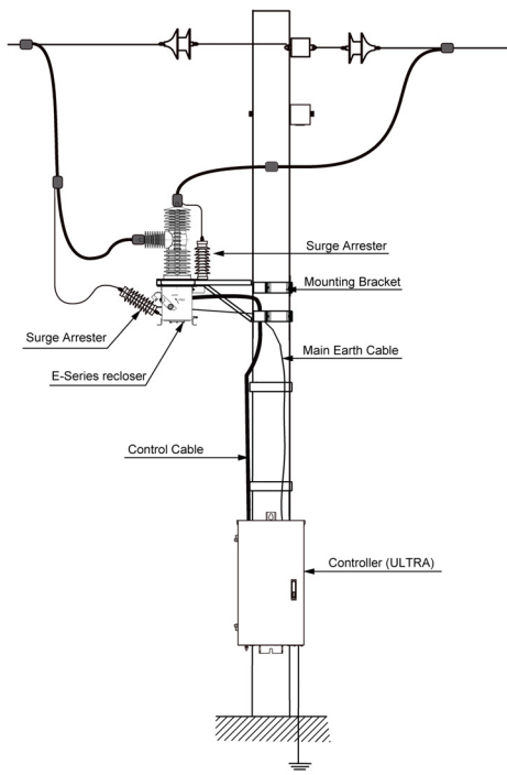
38 kV Center Mounting Example
