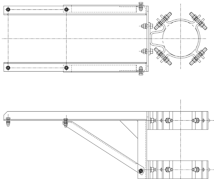
27 kV/38 kV Mounting bracket assembly (Same mounting bracket for end and center mounting)
