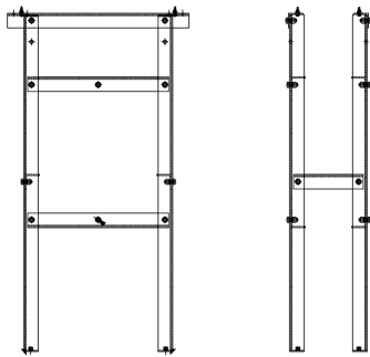
27 kV / 38 kV Substation mounting bracket
