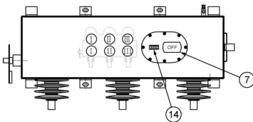
Typical bottom view of E series 27 kV/38 kV switchgear
