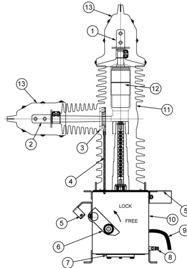
Cross section of E series 38 kV switchgear
