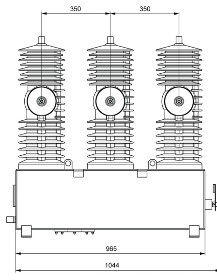
Front view of E-series 38 kV
