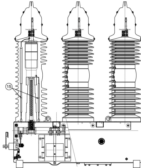
Typical front view of E series 27 kV/38 kV switchgear
