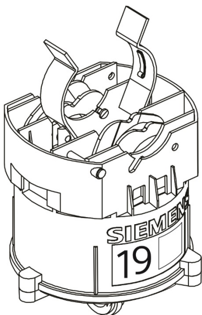
Fig 5. Isometric View
