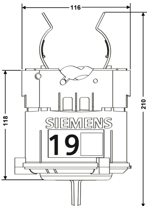
Fig 4. Front View
